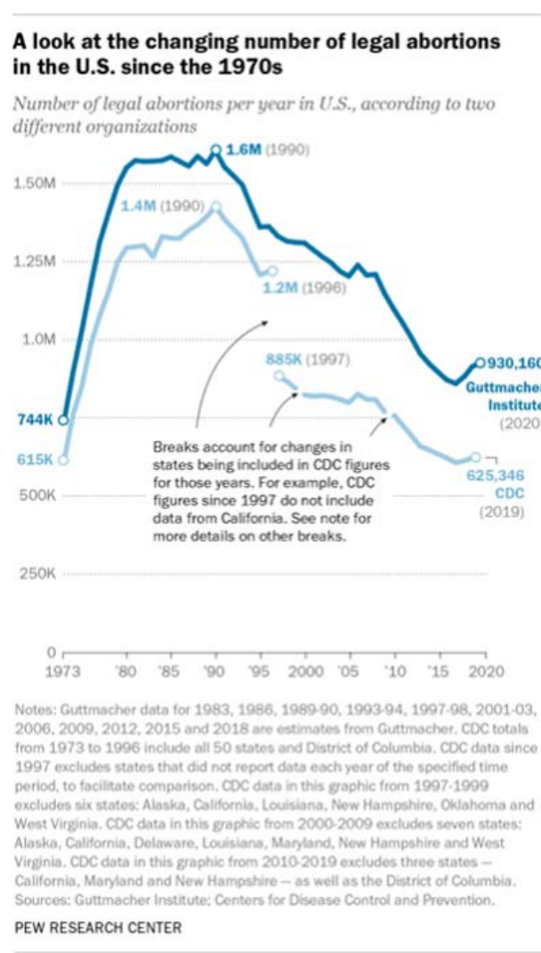
Figure 2: US TABs
